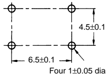
PCB Mounting (Top View)
