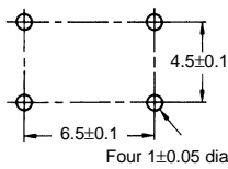
PCB Mounting (Top View)
