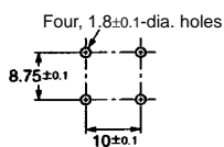
PCB Cutout Dimensions (Bottom View)
