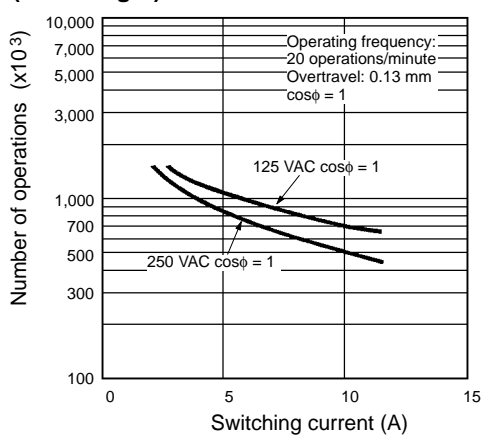
Electrical Life Expectancy (Pin Plunger)
