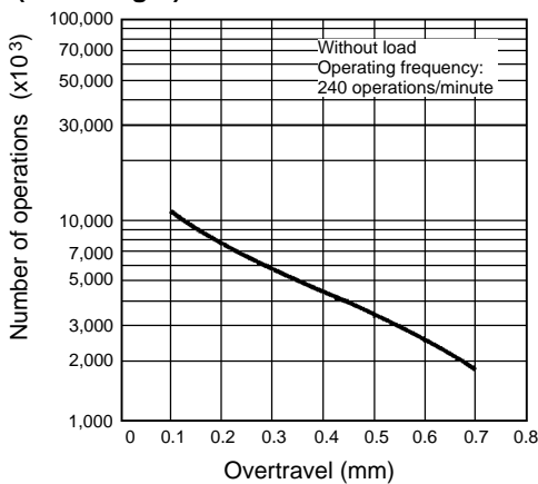
Mechanical Life Expectancy (Pin Plunger)
