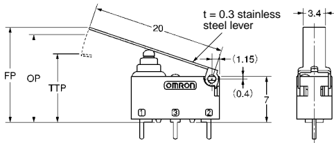
Simulated Hinge Lever D2HW-□23□□
