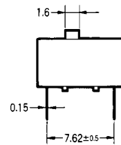
Raised Actuator
