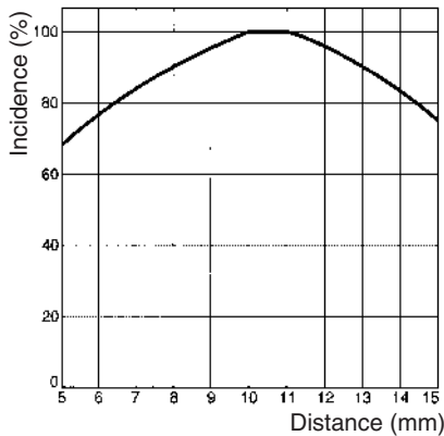
Color Sensing Capacity E3M-VG□□
