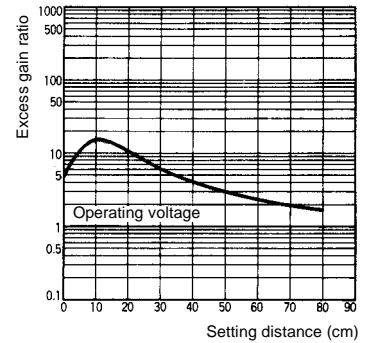
Excess Gain Ratio vs. Setting Distance (Typical) E3JM-DS70j 4(T)
