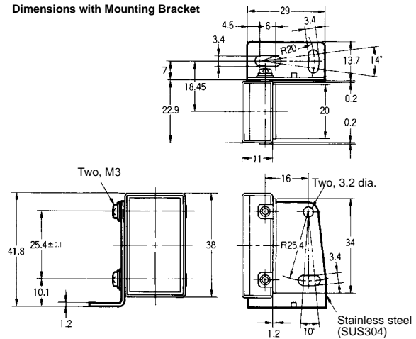
Dimensions with Mounting Bracket
