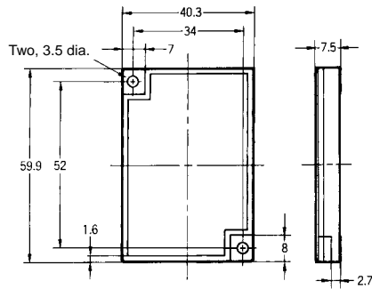
Dimensions with Mounting Bracket
