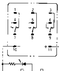
DC Model
